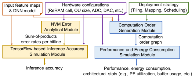
Figure 6: Overview of DL-RSIM [35] simulation framework.
