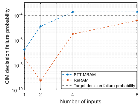
Figure 4: CiM decision failure vs. the number of inputs in STT-MRAM, ReRAM during scouting-based NVM-CiM.
