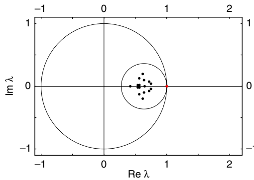
Figure 5. Eigenvalues in the complex plane for inhibitory coupling. The Gershgorin disc, that contacts the unit disc from the inside, contains all eigenvalues of the stability matrices A . The black dots show eigenvalues of a specific stability matrix for a network of N = 16 oscillators (in which every connection is present with probability p = 0.25 ) with coupling strengths \varepsilon_{ij} = \varepsilon/k_i , \varepsilon = -0.2 , \tau = 0.15 and a particular rank order of the perturbation.
