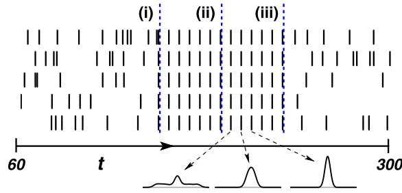
Figure 3. Switching between irregular and synchronous dynamics ( N = 400 , p = 0.2 , I = 4.0 , \varepsilon = -16.0 , \tau = 0.14 ). Firing times of five oscillators are shown in a time window \Delta t = 240 . Vertical dashed lines mark external perturbations: (i) large excitatory pulses lead to synchronous state, (ii) a small random perturbation ( |\Delta\phi_i| \leq 0.18 ) is restored, (iii) a sufficiently large random perturbation ( |\Delta\phi_i| \leq 0.36 ) leads to an irregular state. (Bottom) Time evolution of the spread of the spike times after perturbation (ii), total length \Delta t = 0.25 each. Figure modified from [38].
