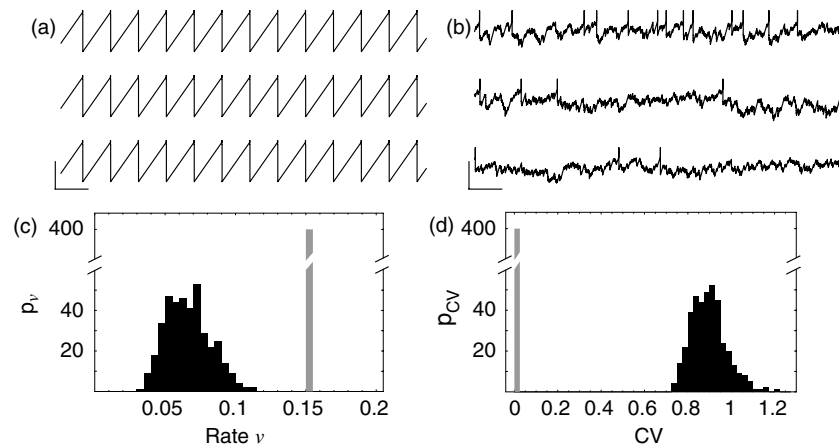
Figure 2. Coexistence of (a) synchronous and (b) irregular dynamics in a random network ( N = 400 , p = 0.2 , I = 4.0 , \varepsilon = -16.0 , \tau = 0.035 ), cf [38]. (a) and (b): trajectories of the potential U(\phi_i) of three oscillators (angular bars: time scale (horizontal) \Delta t = 8 ; potential scales (vertical) (a) \Delta U = 8 , (b) \Delta U = 2 ; spikes of height \Delta U = 1 added at firing times). Distributions (c) p_v of rates and (d) p_{CV} of the coefficient of variation, displayed for the irregular (dark grey) and synchronous (light grey) dynamics. Figure modified from [38].
