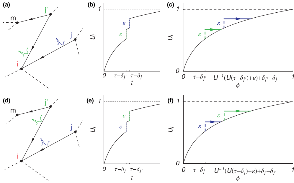
Figure 4. Two signals arriving almost simultaneously induce different phase changes, depending on their rank order. The figure illustrates a simple case where \text{Pre}(i) = \{j, j'\} and \delta_i = 0 . (a)–(c) for \delta_{j'} > \delta_j and (d)–(f) for \delta_j > \delta_{j'} . (a) and (d) Local patch of the network displaying the reception times of signals that are received by oscillator i . Whereas in (a) the signal from j' arrives before the signal of j , the situation in (d) is reversed. (b) and (e) Identical coupling strengths induce identical jumps of the potential U but (c) and (f) the phase jumps these signals induce are different and depend on the order of the incoming signals. For small |\delta_i| \ll 1 , individual phase jumps are encoded by the p_{i,n} .
