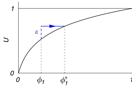
Figure 1. An incoming pulse of strength \varepsilon induces a phase jump \phi_1^+ := \phi_1(t^+) = U^{-1}(U(\phi_1(t)) + \varepsilon) = H_\varepsilon(\phi_1) that depends on the state \phi_1 := \phi_1(t) of the oscillator at time t of pulse reception. Due to the curvature of U , an excitatory pulse ( \varepsilon > 0 ) induces an advancing phase jump. If the incoming pulse puts the potential above threshold ( U(\phi_1) + \varepsilon > 1 ), the phase is reset to zero ( \phi_1^+ = 0 ). An inhibitory pulse ( \varepsilon < 0 ) would induce a regressing phase jump such that the phase may assume negative values (not shown).
