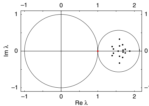
Figure 6. Eigenvalues in the complex plane for excitatory coupling. The Gershgorin disc, that contacts the unit disc from the outside, contains all eigenvalues of the stability matrices A . The black dots show eigenvalues of a specific stability matrix for a network of N = 16 oscillators (in which every connection is present with probability p = 0.25 ) with coupling strengths \varepsilon_{ij} = \varepsilon/k_i , \varepsilon = 0.2 , \tau = 0.15 and a particular rank order of the perturbation.
